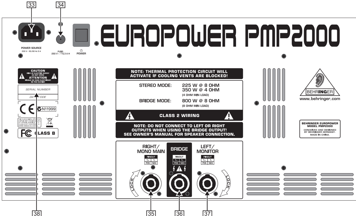
Rear panel connectors
